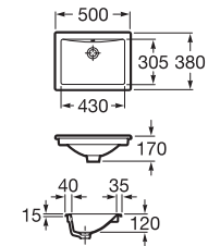
SOFIA-S 枱底盆
