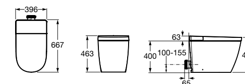
IN-WASH® ONA FLOOR-STANDING P-TRAP 一體式坐地智能座廁
