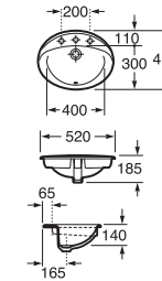
ALOA 枱面盆
