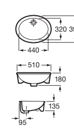
RODEO 枱面盆
